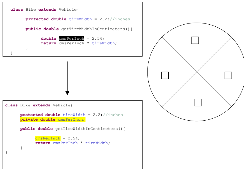
Figure 7.3: A sample training page (top) and a sample recall page (bottom). The refactorings (left, as program code before-and-after refactoring) are the same on both pages. Subjects were instructed to put a check mark in the appropriate direction on the recall page.
